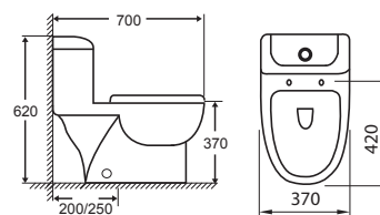
MODEL: BARRY CODE : A388 Washdown One-piece Closet SIZE: 700 x 370 x 620mm S-TRAP: 200mm (White) 250mm (White) Colour: RM 700
