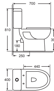
MODEL: MERTON CODE : WD004A CISTERN: CS204 Washdown Pedestal WC SIZE: 700 x 400 x 810mm S-TRAP: 250mm (Roughing-In) P-TRAP: 180mm (Roughing-In) Colour: White RM 700
