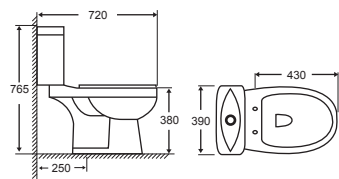
MODEL: HARLO CODE : WD018 CISTERN: CS018 Washdown Pedestal WC SIZE: 720 x 390 x 765mm S-TRAP: 250mm (Roughing-In) P-TRAP: 180mm (Roughing-In) Colour: White RM 550
