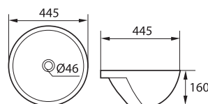
Model: 270A Basin Semi Recesses Size: 445X445X160mm RM 240
