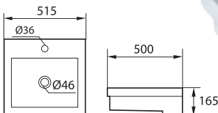
Model: 281 Basin Semi Recesses Size: 515X500X165mm RM 380
