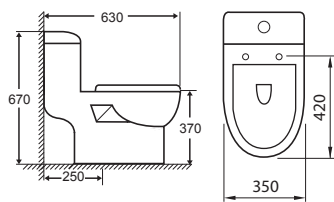
MODEL: HACODA CODE : A888 Washdown One-piece Closet SIZE: 630 x 350 x 670mm S-TRAP: 250mm (White) Colour: RM 700
