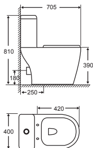
MODEL: ROYAL CODE : WD002A CISTERN: CS204 Washdown Pedestal WC SIZE: 705 x 400 x 810mm S-TRAP: 250mm (Roughing-In) P-TRAP: 180mm (Roughing-In) Colour: White RM 800
