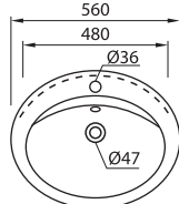
MODEL: 201 Above Counter Basin Size: 560 x 485 x 200mm
