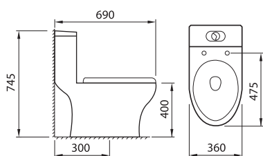
OXFORD CODE : A893 Siphonic One-piece Closet SIZE: 690 x 360 x 745mm S-TRAP: 300mm (White) Colour: RM 850
