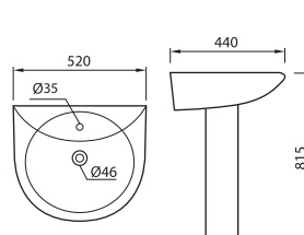
MODEL: SANTA CODE: B510(Basin) / BP510(Pedestal) Dimensions (mm): 520W x 440L x 815H
