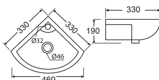
MODEL: NATAL CODE: B310C Dimensions (mm): 330W x 330L x 190H
