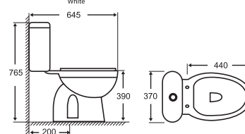
MODEL: LUTON CODE : WD012 CISTERN: CS012 Close-coupled Washdown Pedestal WC SIZE: 645 x 370 x 440mm S-TRAP: 200mm (Roughing-In) P-TRAP: 180mm (Roughing-In) Colour: White RM 500
