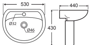
MODEL: FORTUNE CODE: B301/HP301 Dimensions (mm): 530W x 440L x 430H
