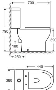
MODEL: EPSON CODE : WD014 CISTERN: CS014 Washdown Pedestal WC SIZE: 700 x 380 x 790mm S-TRAP: 250mm (Roughing-In) P-TRAP: 180mm (Roughing-In) Colour: White RM 750
