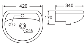
MODEL: TOTO CODE: B304 Dimensions (mm): 420W x 340L x 170H
