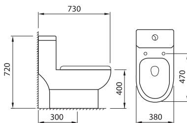
MODEL: NITRON CODE : A886 Siphonic One-piece Closet SIZE: 730 x 380 x 720mm S-TRAP: 300mm (White) Colour: RM 850
