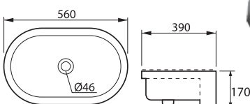
Model: 294E Basin Semi Recesses Size: 560X390X170mm RM 320
