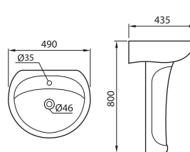
MODEL: HUIDA CODE: B511(Basin) / BP511(Pedestal) Dimensions (mm): 490W x 435L x 800H
