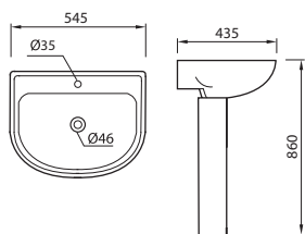
MODEL: PRESTON CODE: B201(Basin) / BP510(Pedestal) Dimensions (mm): 545W x 435L x 860H
