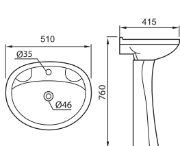
MODEL: CEARA CODE: B206(Basin) / BP206(Pedestal) Dimensions (mm): 510W x 415L x 760H
